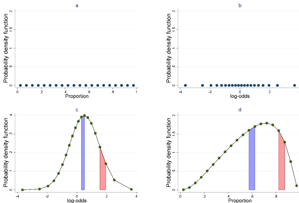
Appendix Figure 1: Illustration of how to plot the modelled distribution from a mixed effects logistic regression on the proportion scale. Full details are given in the text.
