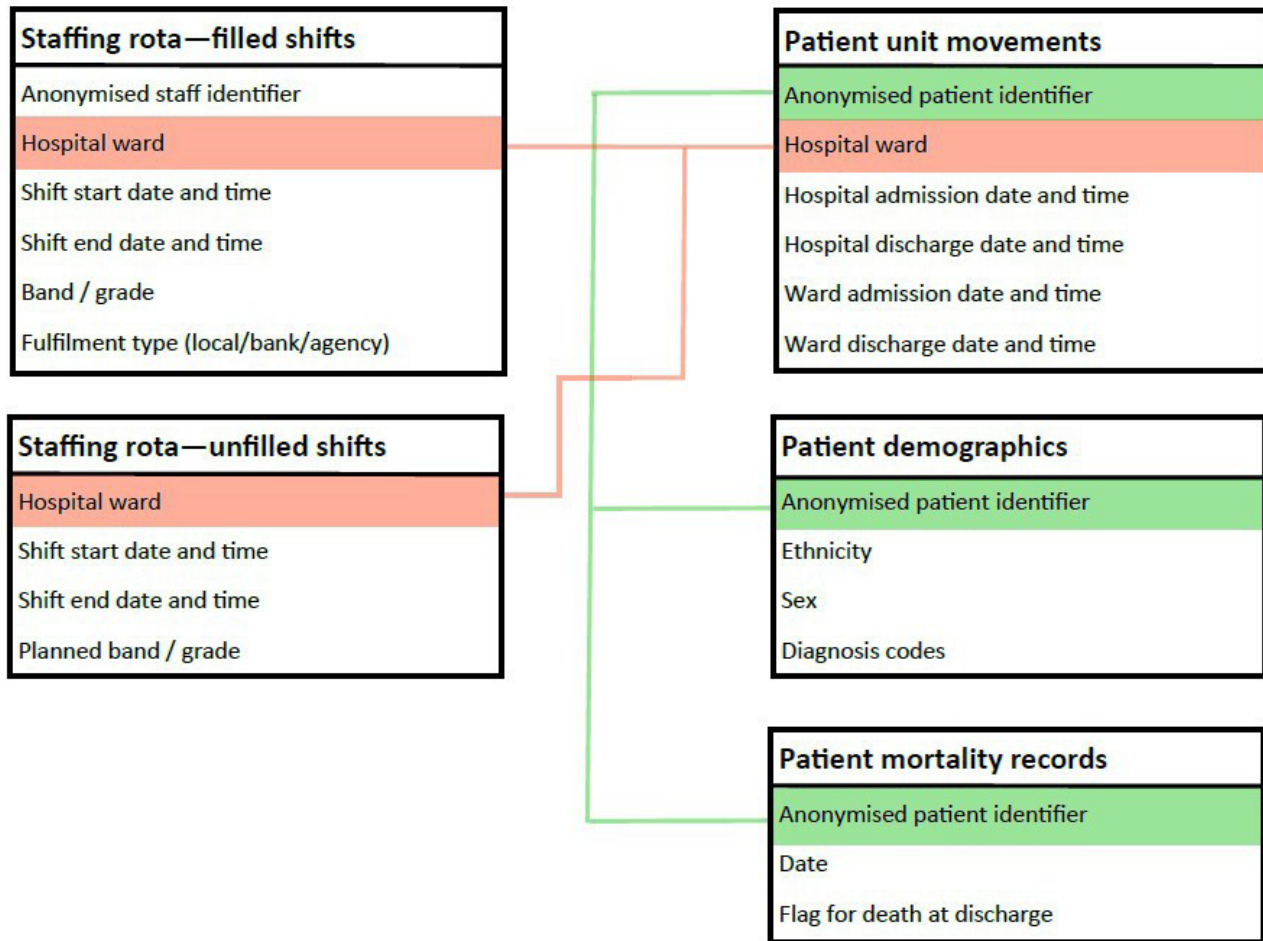
Figure 1 Data structure.
